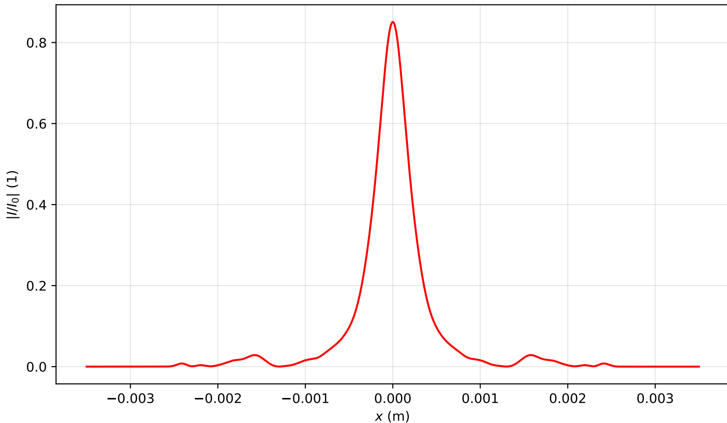
Intensity profile I(x, y = 0, z = 3.344)/I_0 , P_{in}=3.5P_{cr} , artificial time
